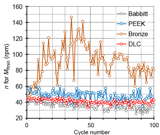
Fig. 8 Comparison of shaft speed (rpm), at which minimum friction torque was measured.
