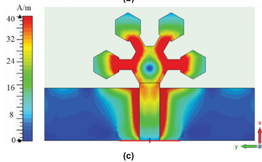
FIGURE 12. (a) Prototype of fractal butterfly antenna [1], (b) snowflake-shaped dual-beam wideband antenna prototype, and (c) snowflake-shaped dualbeam antenna surface current distribution [15].
