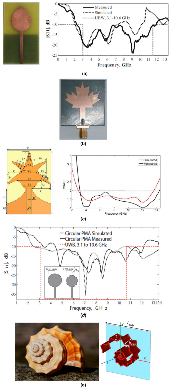
FIGURE 5. (a) Orchid petal shaped UWB antenna and its simulated reflection coefficient [31], (b) prototype of a maple leaf shaped UWB antenna [32], (c) 5 Volume xx Palmate-leaf-shaped radiator and its VSWR graph [3], (d) Reflection coefficient of Jasmine flower shaped monopole antenna proposed in [33], and (e) Picture of a button snail modulus (spiral seashell), the basis for a bio-inspired spiral shell dielectric resonator antenna (DRA) at sub-6 GHz, hDRA=29mm [37].
