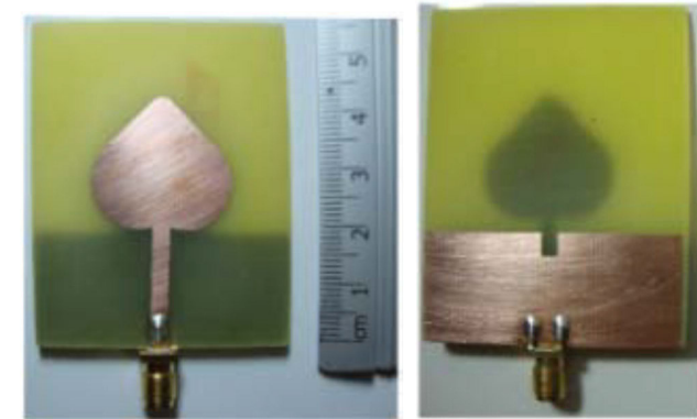
FIGURE 11. Cotton leaf-shaped printed monopole antenna (a) The top side and (b) Lower side of the fabricated antenna [61].
