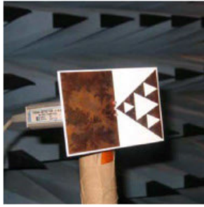
FIGURE 10. Modified Sierpinski Fractal Gasket physical model [60].
