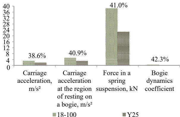
Fig. 5. Comparative analysis of the tank car dynamics when using the 18-100 and Y25 bogies
