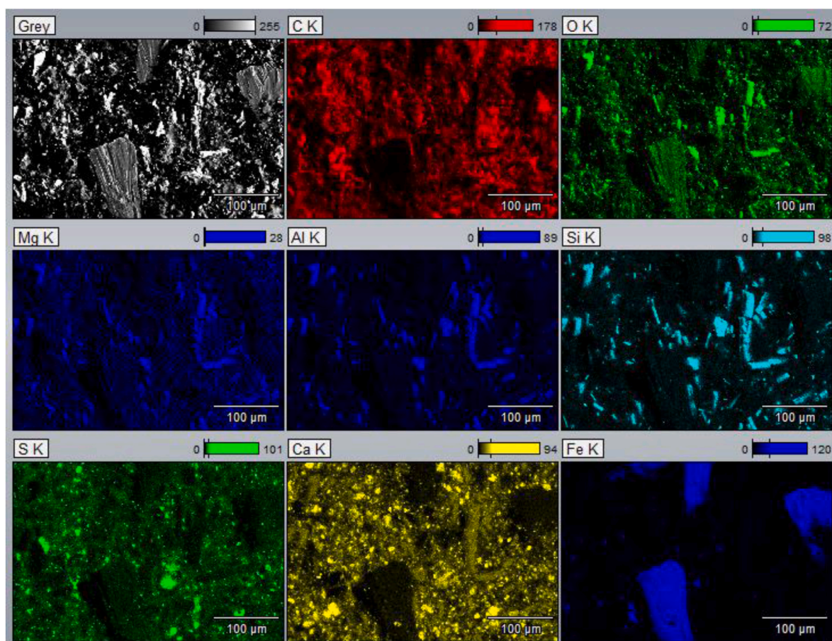
Fig. 1. EDX maps of the original friction surface of the pin sample M_{\text{RNPF/NBR}} .
