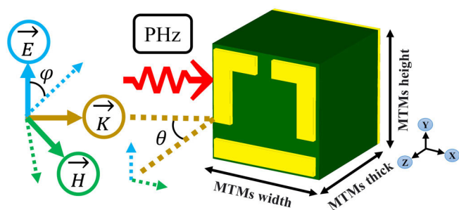
Fig. 1. Structural design and incident field directions of a perfect absorber.
