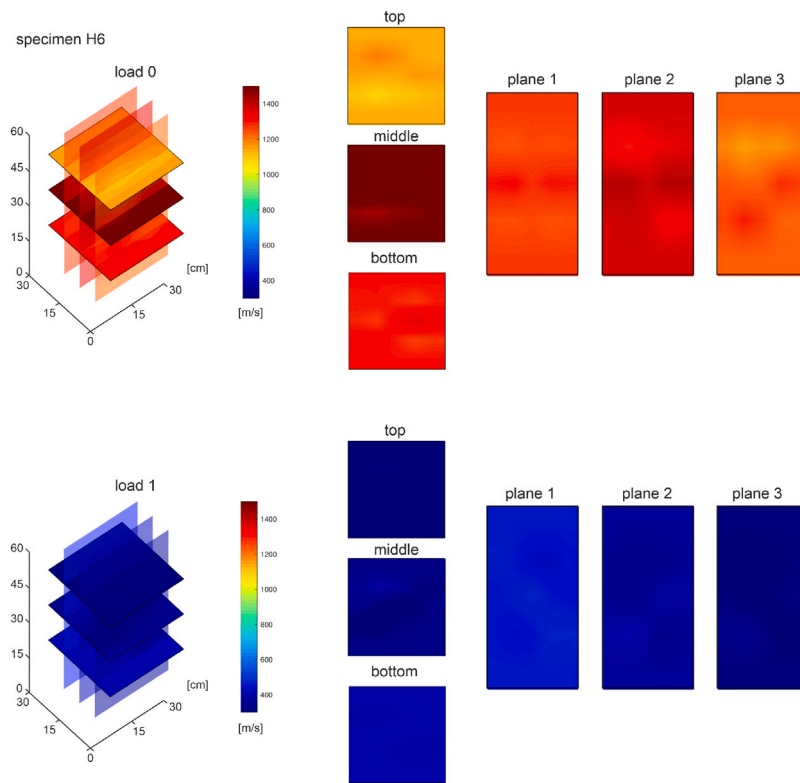
Fig. 17. Results from sonic tomography (specimen H6).
