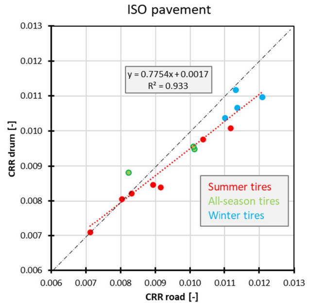
Fig. 8 Comparison of results obtained on the smooth ISO pavement and its replica ISO-dr. Drum results with flat correction according to Eq. 1
