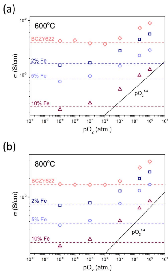
Fig. 6 Total electrical conductivity as a function of oxygen partial pressure measured at 600 °C (a) and 800 °C (b) for BaCe_{0.6}Zr_{0.2}Y_{0.18}Fe_{0.02}O_{3-\delta} (2% Fe), BaCe_{0.6}Zr_{0.2}Y_{0.15}Fe_{0.05}O_{3-\delta} (5% Fe), BaCe_{0.6}Zr_{0.2}Y_{0.1}Fe_{0.1}O_{3-\delta} (10% Fe), and BCZY622. 26
