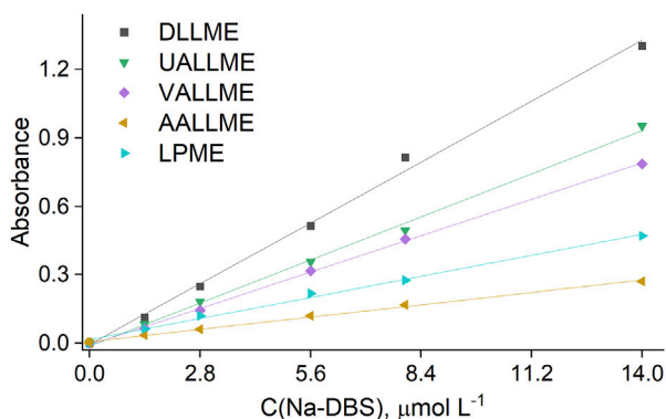
FIGURE 8 Calibration curves for the determination of anionic surfactants with CV, obtained by different extraction procedures.
