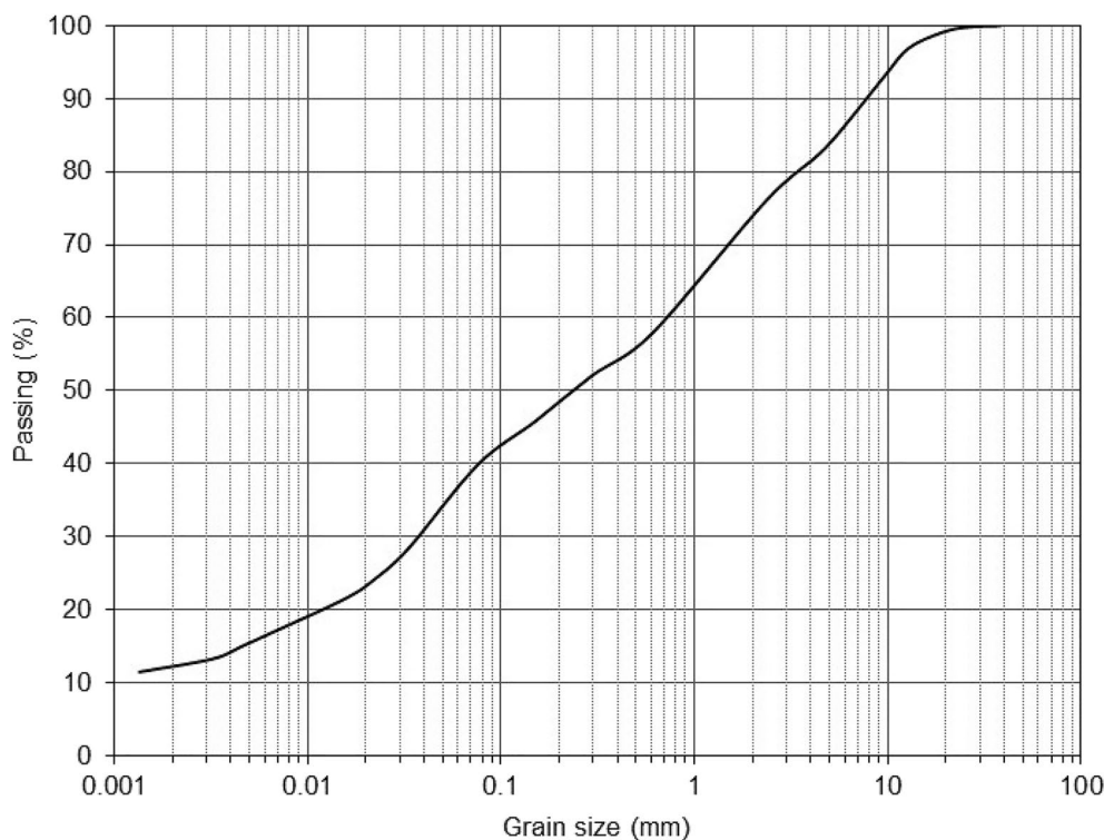
Figure 1. Grain-size distribution plot for the clayey sand soil.
