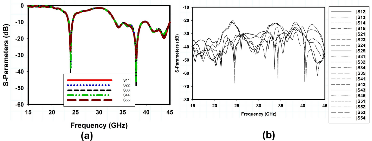
Fig. 11. Proposed reflective metasurface based MIMO antenna: (a) reflection coefficients, (b) mutual coupling between the MIMO antenna elements.
