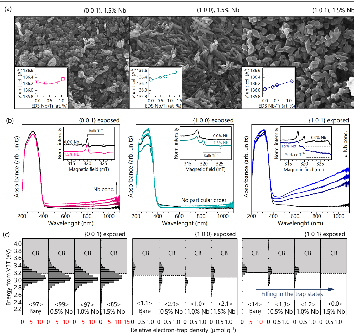
Figure 13.1. Exemplary SEM images of the TiO 2 nanoparticles doped with 1.5% atomic of Nb (relative to Ti), with observed evolution of the anatase unit cell volume for each series in the inset (a). Absorbance spectra of all obtained Nb-doped samples, together with the EPR spectra (77 K) of the corresponding unmodified and most-doped samples in each series shown in the inset (b). Distribution of the electron-trap density obtained for all samples from the RDB-PAS measurements. Please note different values on the X scales. Total trap densities are given in chevrons within each individual graph (c). The “VBT” stands for “valence band top” and “CB” stands for “conduction band”.
