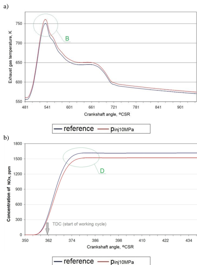
Fig. 9. Patterns of trends in: temperature of exhaust gas T_{\text{exh}} , for part of engine cycle and with marked highest incidence of the highest amount of the difference of temperature B (a); and concentration of \text{NO}_x particles and with marked highest appearance of the highest amount of the difference of concentration of \text{NO}_x particles D (b), derived as a product of numerical modeling of working process of engine regarding the introduced modifications in opening pressure of injector p_{\text{inj}} [38]
