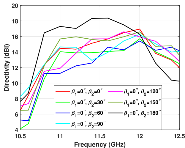
FIGURE 10. Directivity with the variation in frequency for different orientations of BSM-2.
