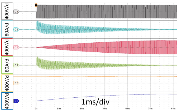
Fig. 16. Classic DAB starting procedure based on SPS. From top: C1 – primary phase voltage, C2 – primary phase current, C3 – secondary phase voltage, C4 – secondary phase current, C5 – input supply DC voltage, C6 – output DC voltage
