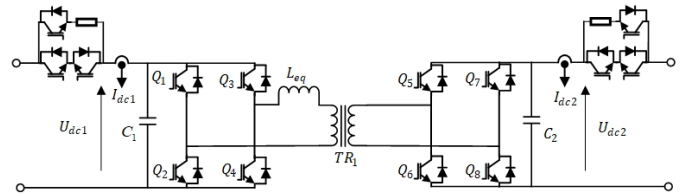
Fig. 7. DAB with hardware soft start resistors
