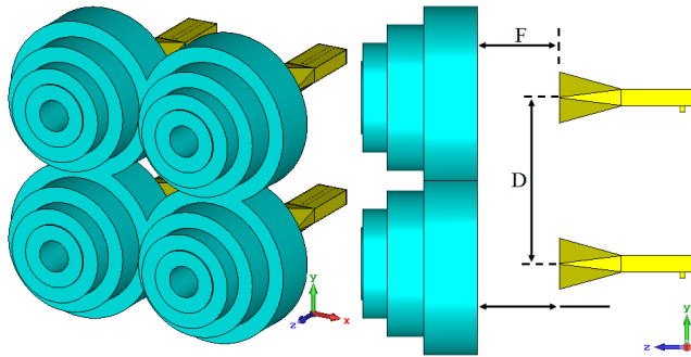
FIGURE 8. Configurations of monopulse dielectric lens antenna.
