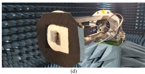
FIGURE 14. (a) top view of the proposed horn array antenna, photos of the fabricated (b) disassembled and (c) assembled horn array antenna and (d) the measurement setup inside the anechoic chamber.
