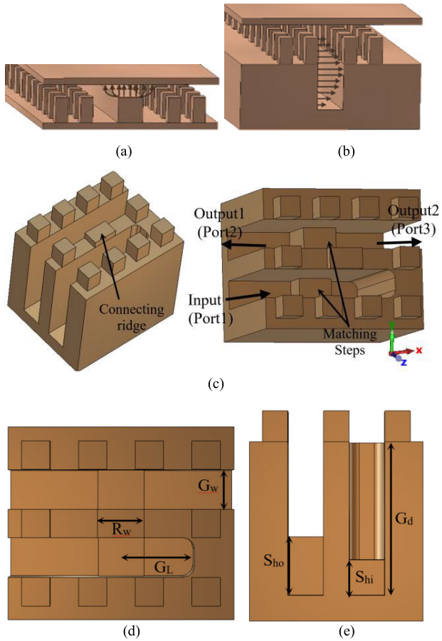
FIGURE 1. Geometries of the (a) ridge gap waveguide and (b) E-plane groove gap waveguide, and (c) perspective, (d) top and (e) side views of the proposed power divider.
