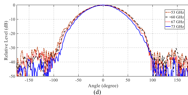
FIGURE 16. The simulated (a) E-plane and (b) H-plane normalized radiation patterns of the horn array antenna and the measured (c) E-plane and (d) H-plane ones.
