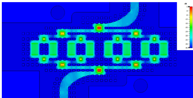
FIGURE 12. The electric field distribution on the back-to-back power divider structure.
