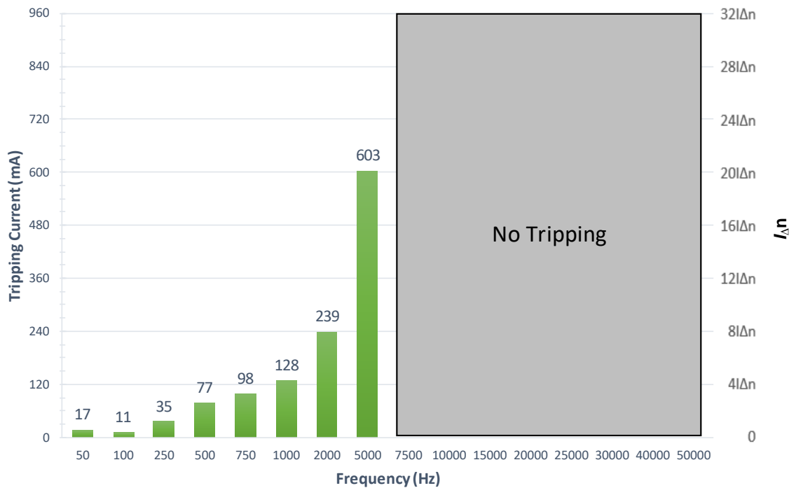
Figure 53: Test results of F-type (30 mA) RCD (RCD_F2) for the following slowly rising residual currents: (A) test results from DC (0 Hz) to AC 45 Hz, (B) test results from 50 Hz to 50000 Hz.
