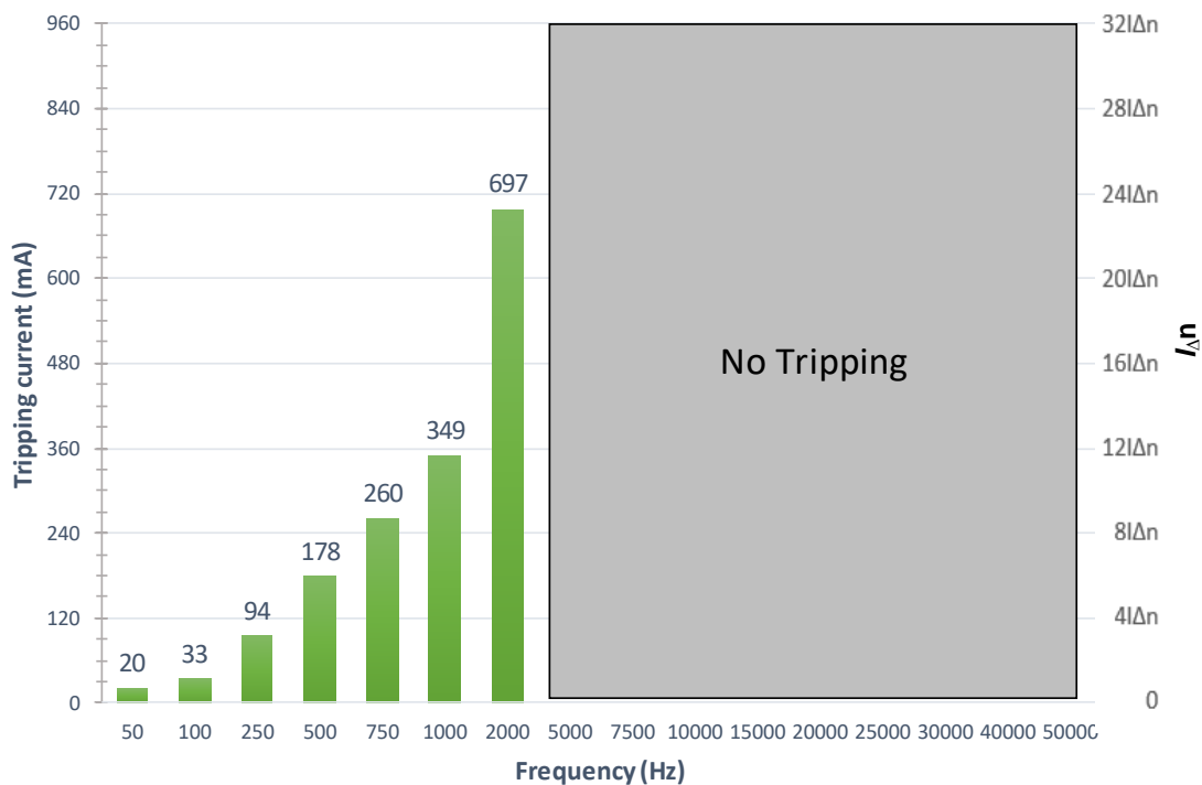
Figure 52: Test results of F-type (30 mA) RCD (RCD_F1) for the following slowly rising residual currents: (A) test results from DC (0 Hz) to AC 45 Hz, (B) test results from 50 Hz to 50000 Hz.
