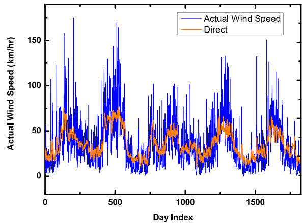
(b) LSTM-based direct training results
