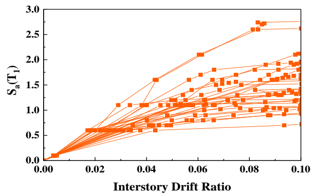
Figure 4: IDA curve of the 4-story structure having soil D including near field pulse like records.
