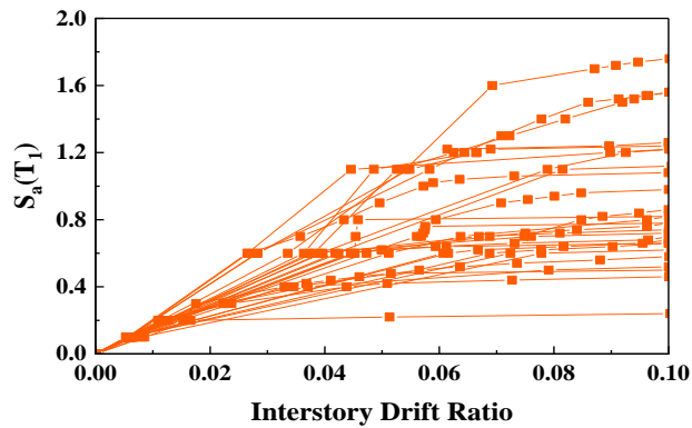
Figure 5: IDA curve of the 6-story structure having soil D including near field pulse like records.
