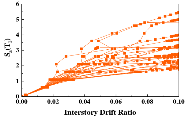
Figure 3: IDA curve of the 2-story structure having soil D including near field pulse like records.
