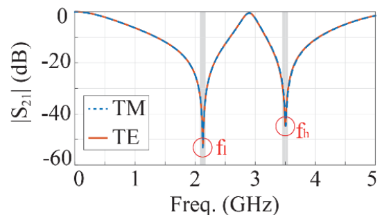
FIGURE 3. Simulated transmission coefficient |S_{21}| (dB) response at normal incidence for TE and TM polarization.
