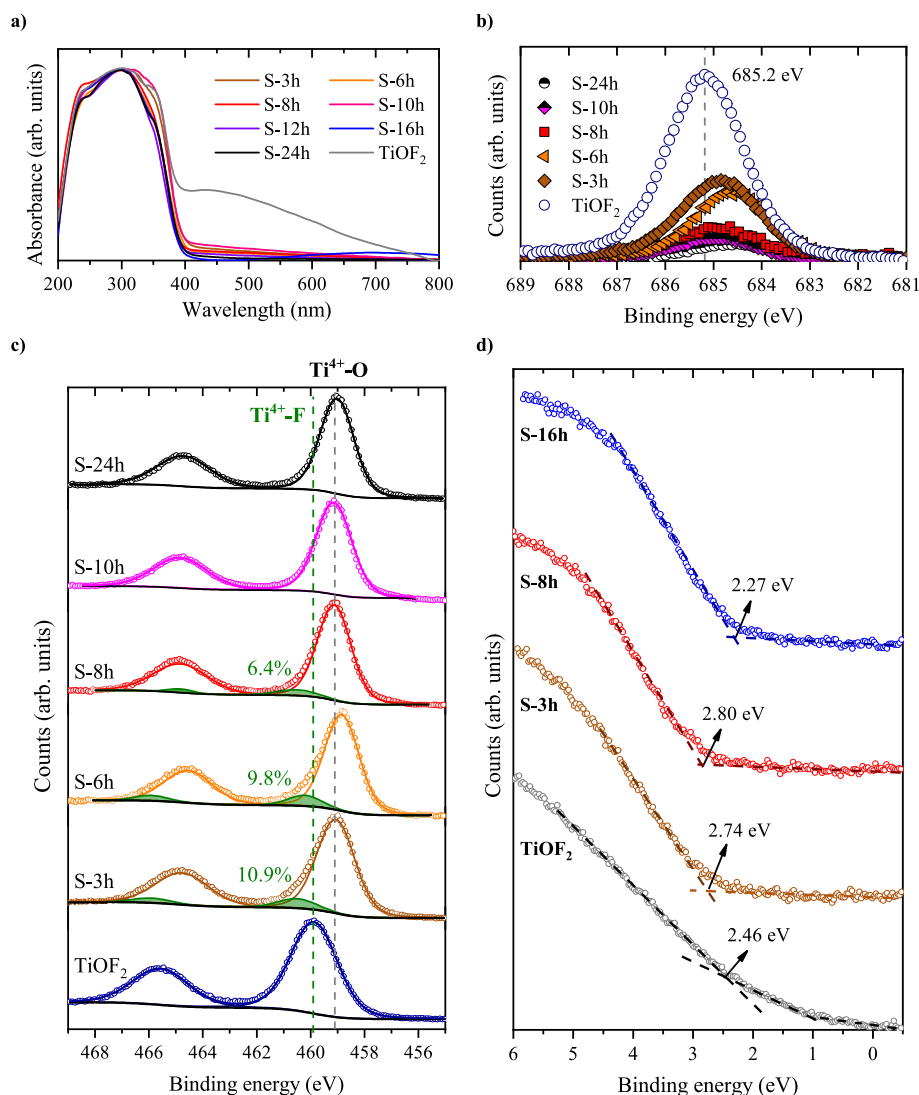
Fig. 3. a) DR/UV-vis absorption spectra of the photocatalysts, b) F1s and c) Ti2p orbital XPS spectra recorded on selected samples from the TiO 2 /TiOF 2 series, d) VB-XPS spectra of selected photocatalysts.
