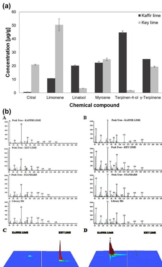
Fig. 1. (a) Concentrations of selected terpenes in Kaffir and Key limes juices. (b) Data obtained from GC×GC-TOF-MS analysis: A , citral mass spectrum, B , terpinen-4-ol mass spectrum, C , 3D chromatograms for citral (selected masses: 41, 69, 84, 94), D , 3D chromatograms for terpinen-4-ol (selected masses: 43, 77, 93, 111).
