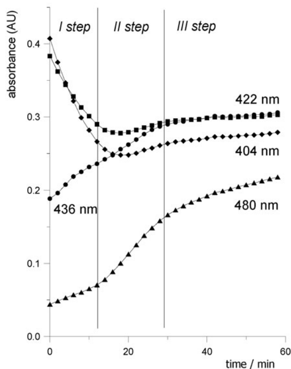
Figure 3. Time dependence of the absorbance at 404, 422, 436 and 480 nm during the incubation of 10^{-4} M 2-hydroxyacridinone with equimolar amount of H_2O_2 and 0.01 \mu\text{g/ml} of HRP.
