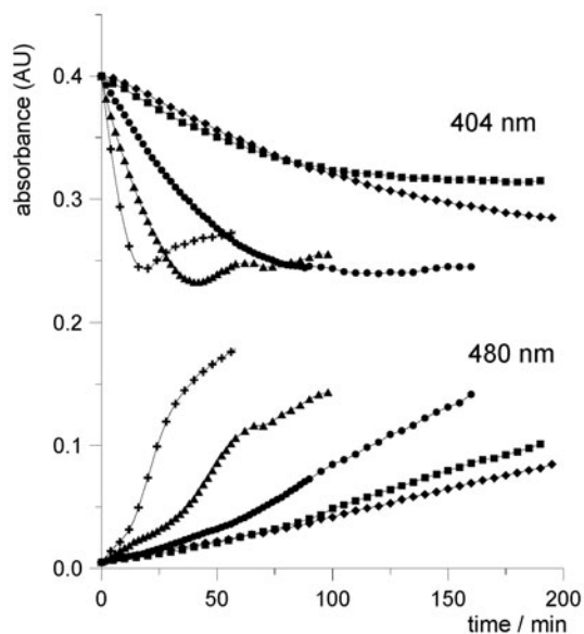
Figure 2. Time dependence of the absorbance at 404 and 480 nm during the incubation of 10^{-4} M 2-hydroxyacridinone with equimolar amount of H_2O_2 and various HRP concentrations: + 0.01 \mu\text{g/ml} ; \blacktriangle 0.005 \mu\text{g/ml} ; \bullet 0.002 \mu\text{g/ml} ; \blacksquare 0.001 \mu\text{g/ml} and \blacklozenge 0.0005 \mu\text{g/ml} .
