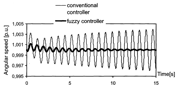
Fig. 4.2b. Angular speed response for a 5% step change of infinite bus voltage. P_g=0.85 [p.u.], Q_g=0.2 [p.u]. Both controllers without PSS
