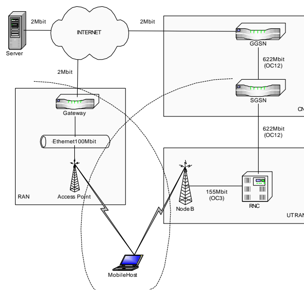
Figure 1. Simulated network architecture
