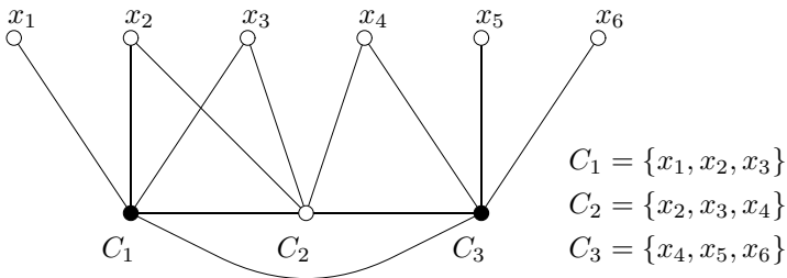
Fig. 1. Split graph
